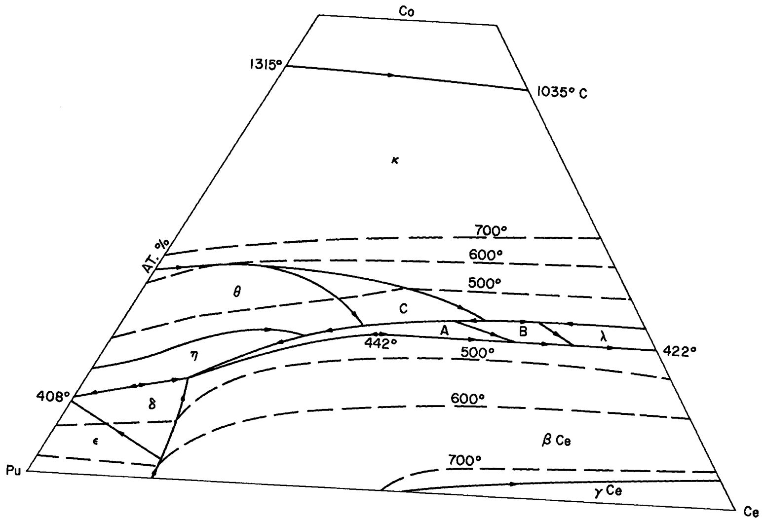
Fig. 4.5. Portion of Pu-Co-Ce Phase Diagram
