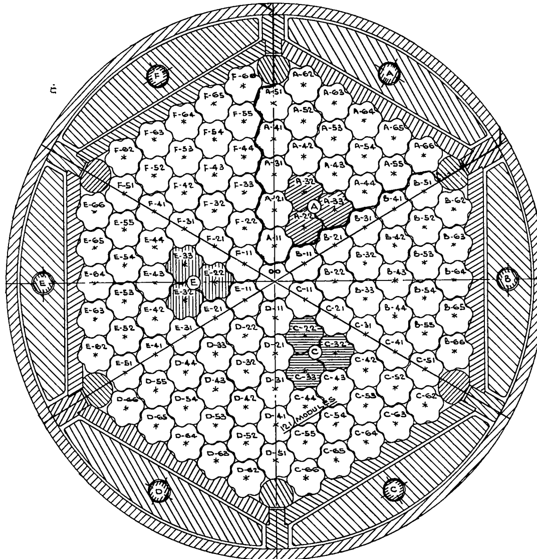
Fig. 5.2. Core Cross Section Used for Nuclear Design
