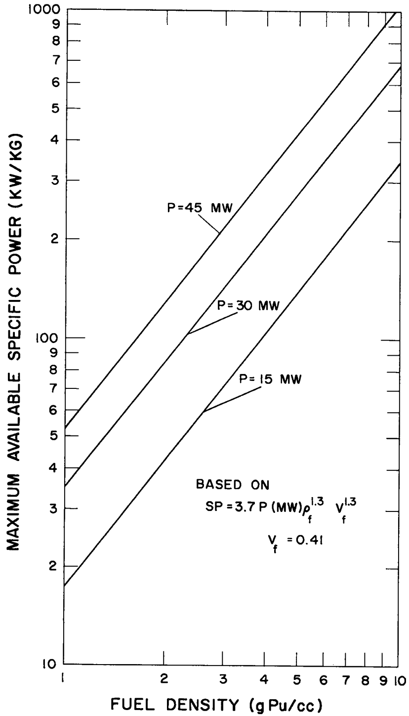
Fig. 3.2. Maximum Specific Power as a Function of Pu Density, Assuming Power Limited Operation
