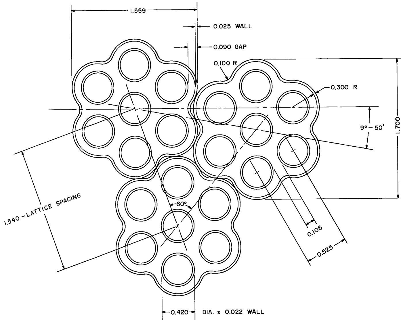
Fig. 5.1. Seven-Pin Corrugated Subassembly
