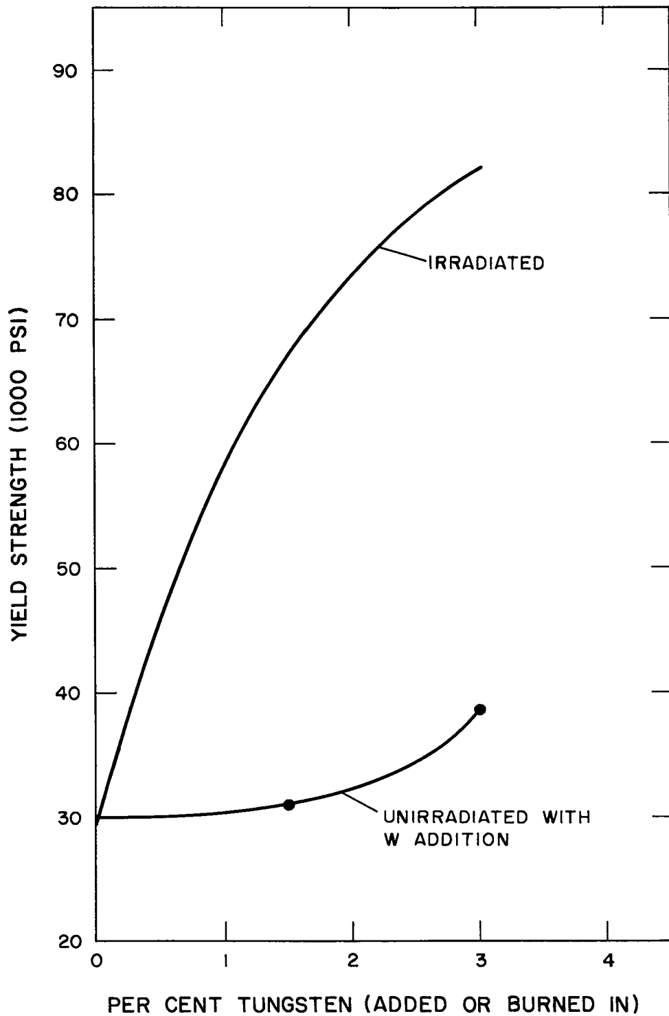
Fig. 4.3. Room Temperature Yield Strength of Irradiated Ta
