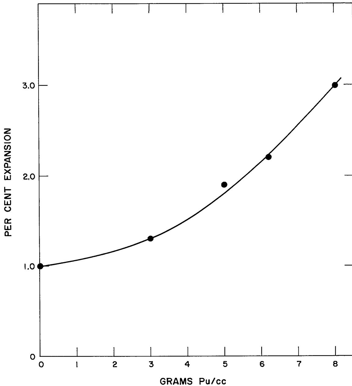
Fig. 4.1. Per Cent Expansion of Some Pu-Co-Ce Alloys on Freezing
