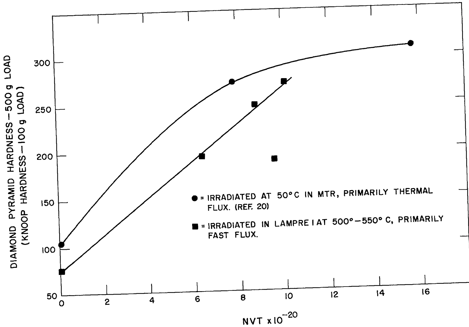
Fig. 4.4. Irradiated Hardness of Ta
