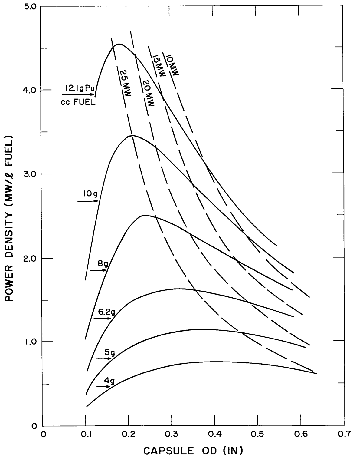
Fig. 3.3. Potential Power Density for MPBE Cores
