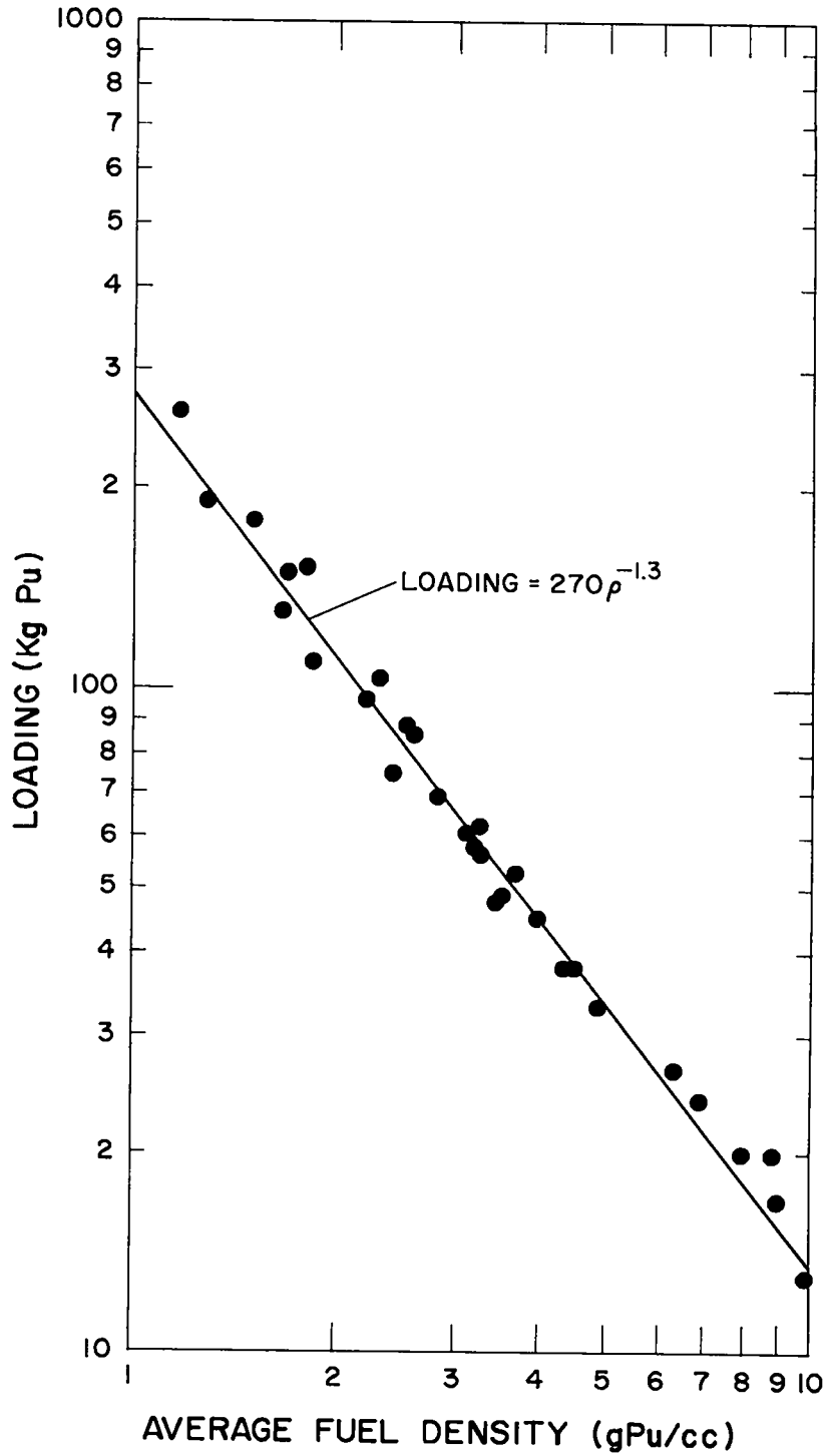
Fig. 3.1. Critical Loadings for Various Molten-Pu-Fueled Cores
