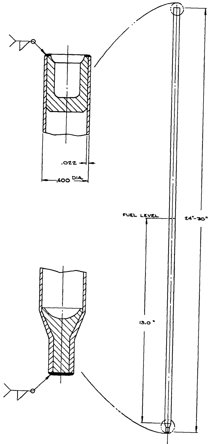
Fig. 4.6. MPBE Fuel Capsule Design
