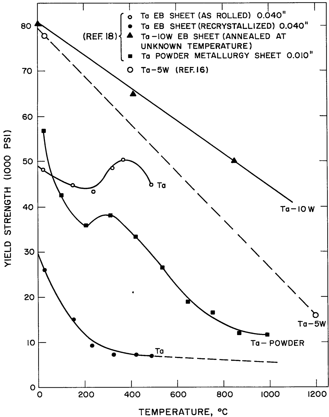
Fig. 4.2. Yield Strength (0.2% Offset) vs Temperature for Ta and Some Ta-5W Alloys
