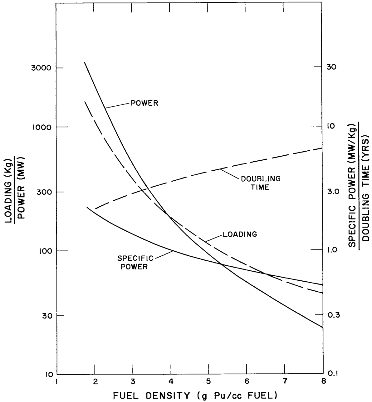
Fig. 7.2. Estimated Performance Factors - Reduced Parasitic Loss
