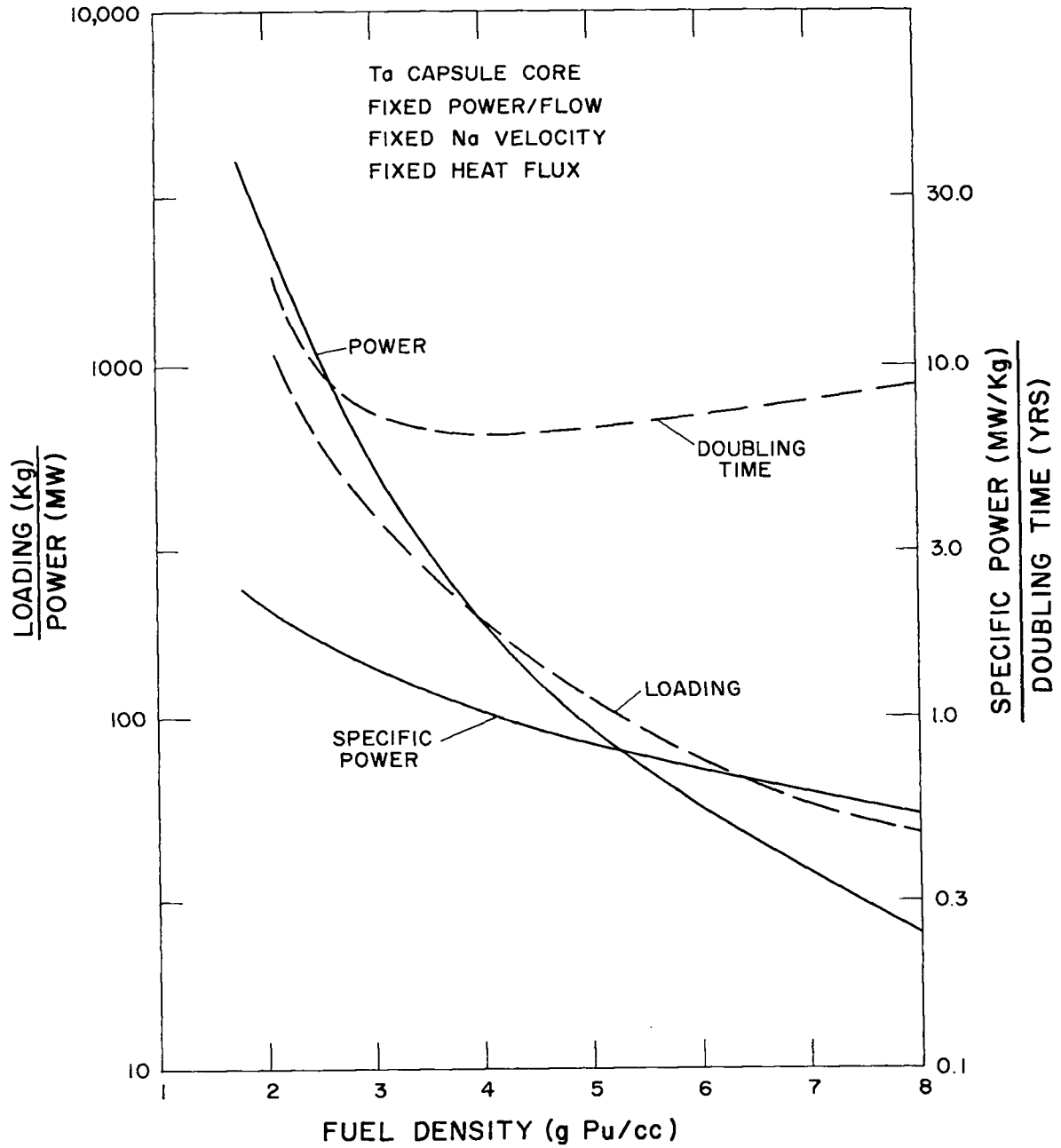
Fig. 7.1. Estimated Performance Factors - Large Molten-Pu-Ta Cores
