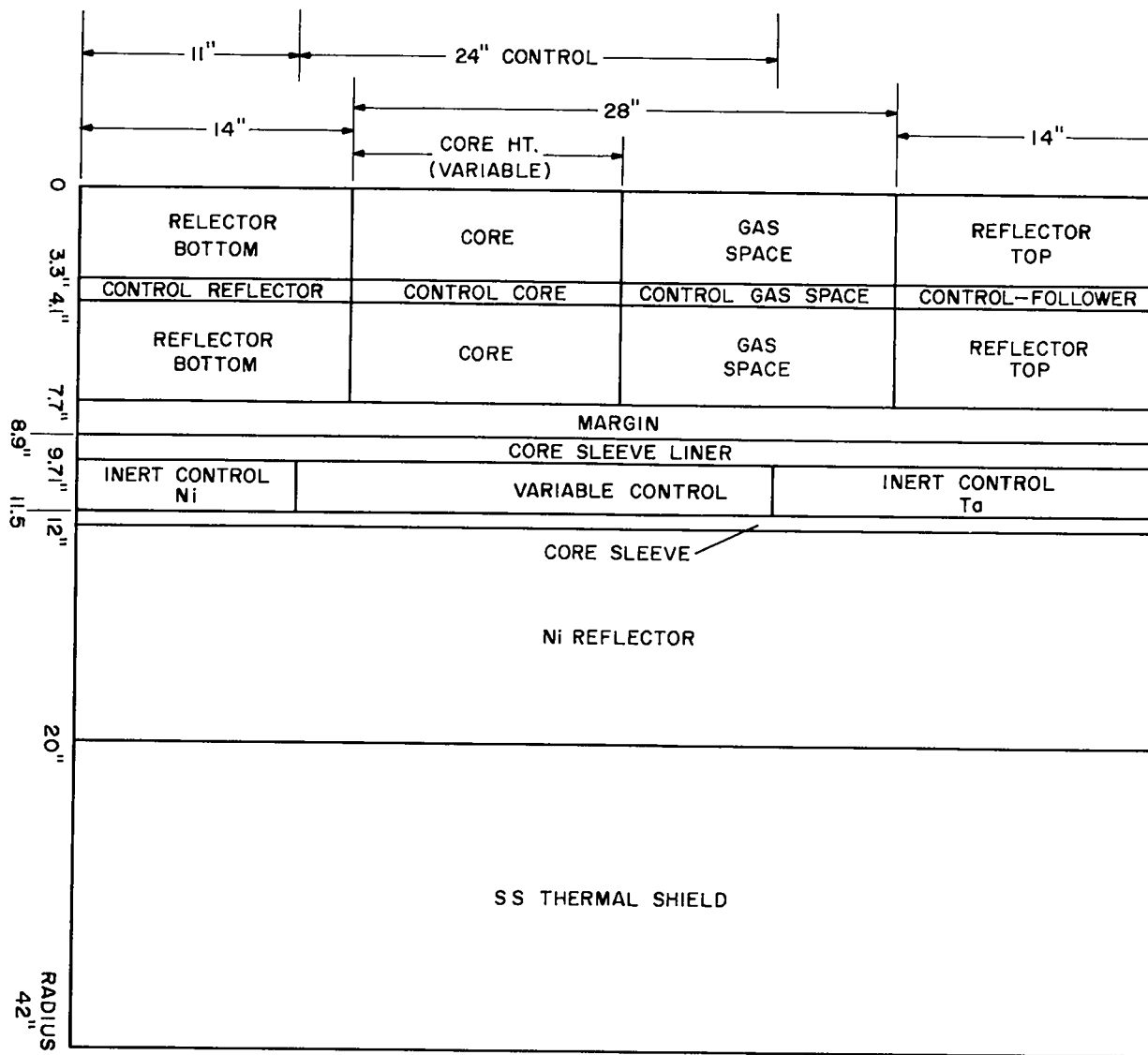
Fig. 5.4. MPBE Calculational Region Layout
