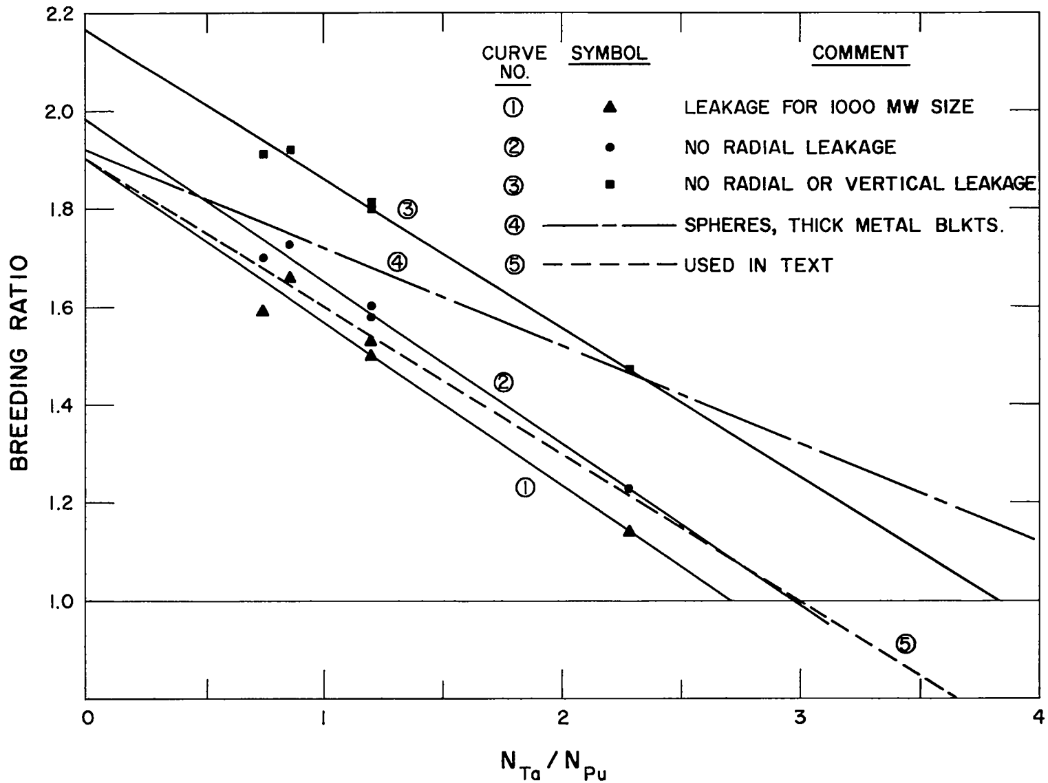
Fig. 2.2. Breeding Ratio as a Function of the Ratio of Ta to Pu Atoms
