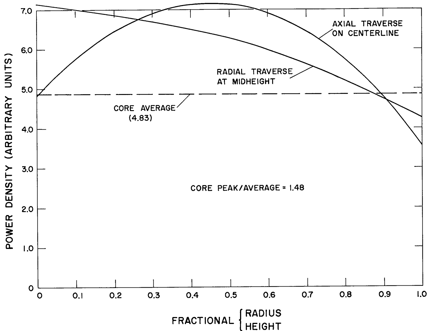
Fig. 6.1. MPBE Power Distributions
