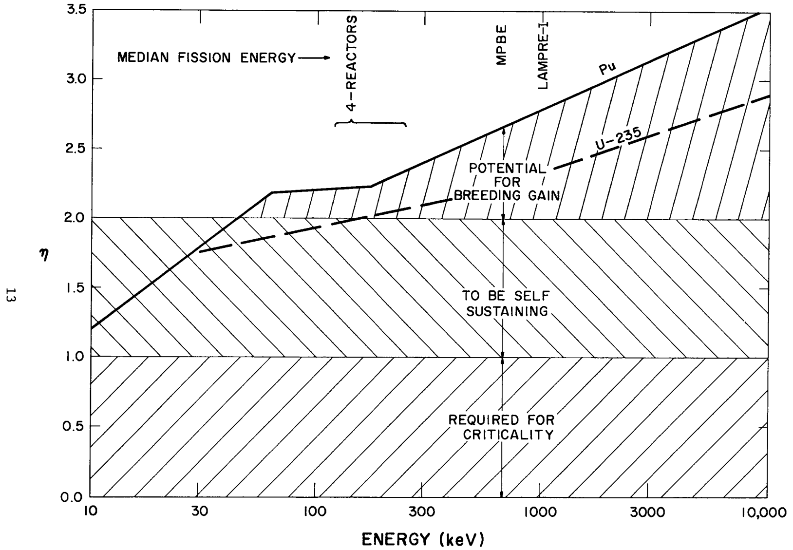
Fig. 2.1. Trend of \eta(E) with E
